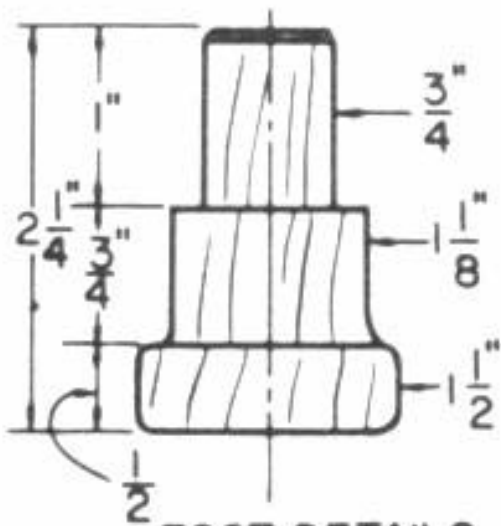
FOOT DETAILS
