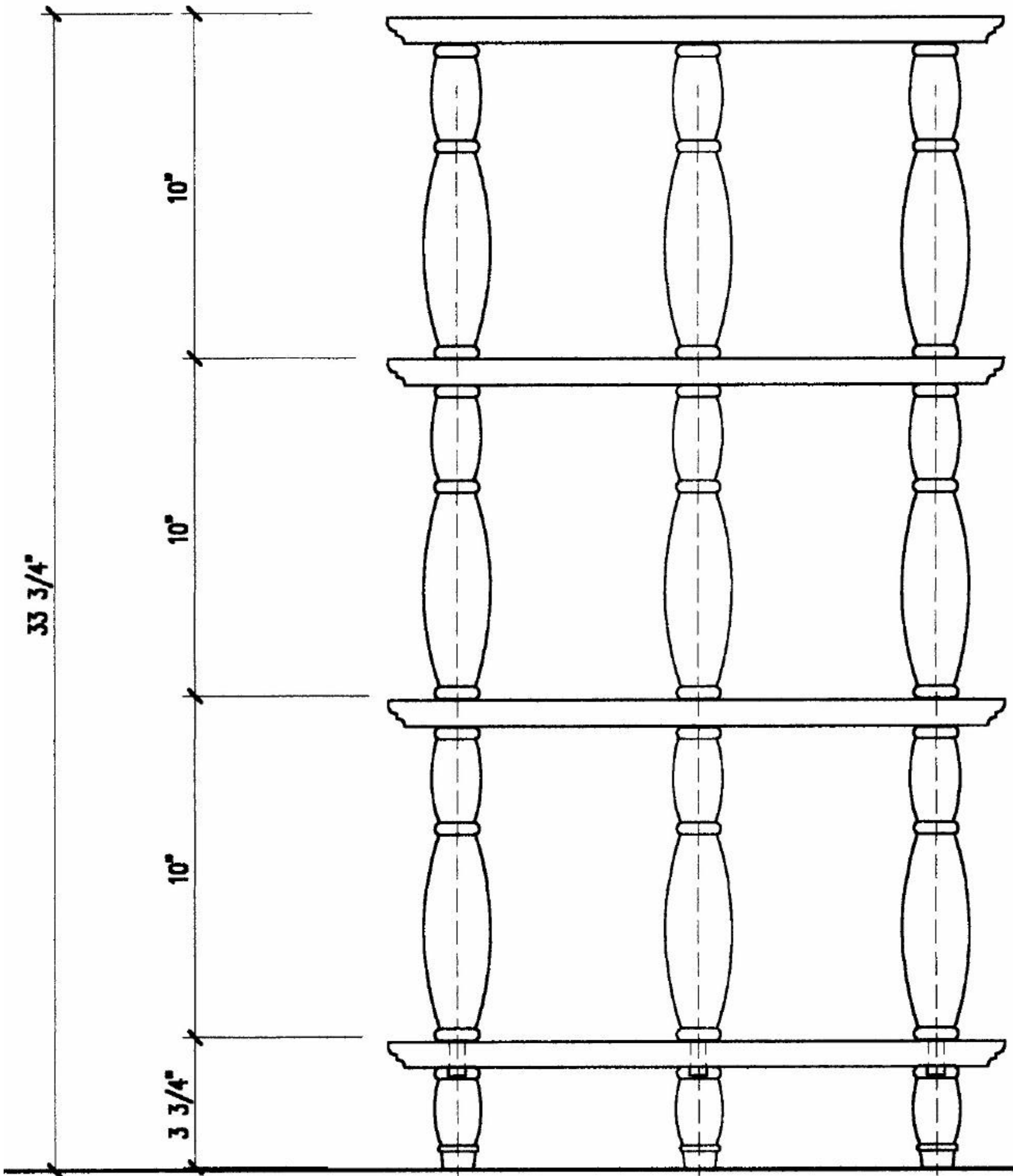
ELEVATION OF CORNER SHELF
