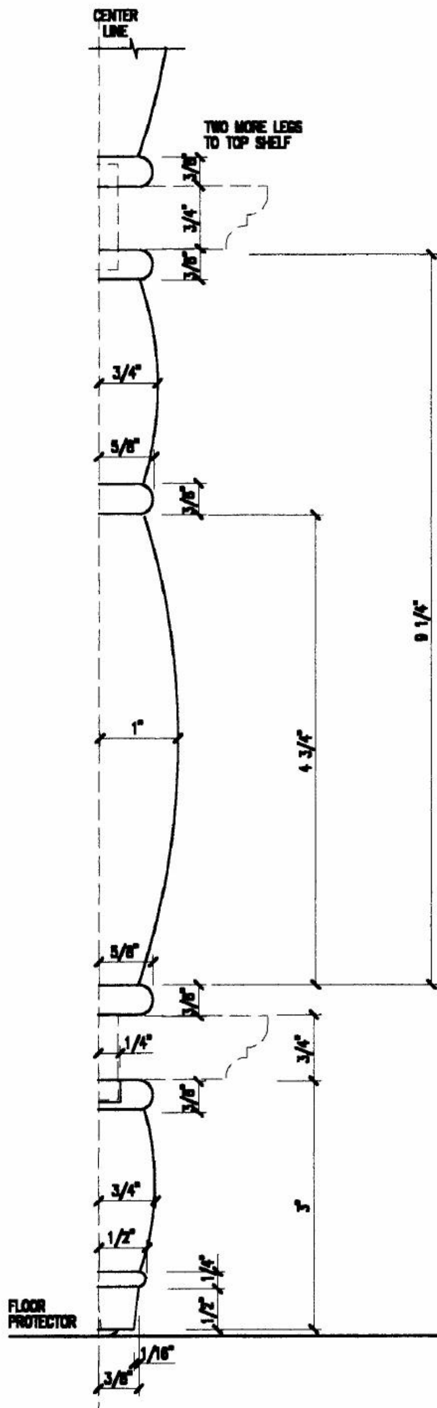
LEG DETAIL OF CORNER SHELF
