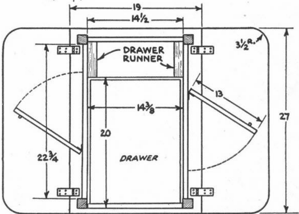
PLAN VIEW (UNDER TOP)
